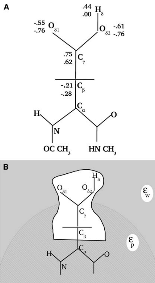
FIGURE 1 (A) Schematic representation of the model compound (2 N -acetyl-1 N -methyl-aspartic acid 1-amide), showing the partial charges at the ionized ( bottom ) values and protonated state ( top ) values. Charges unaffected by ionization are not shown. (B) Schematic view of the titrating side chain, surrounded by the protein ( hatched ) and solvent ( shaded ) dielectric media. Fragment A corresponds to the inner, white region (see “Decomposing the free energy into two components”).
